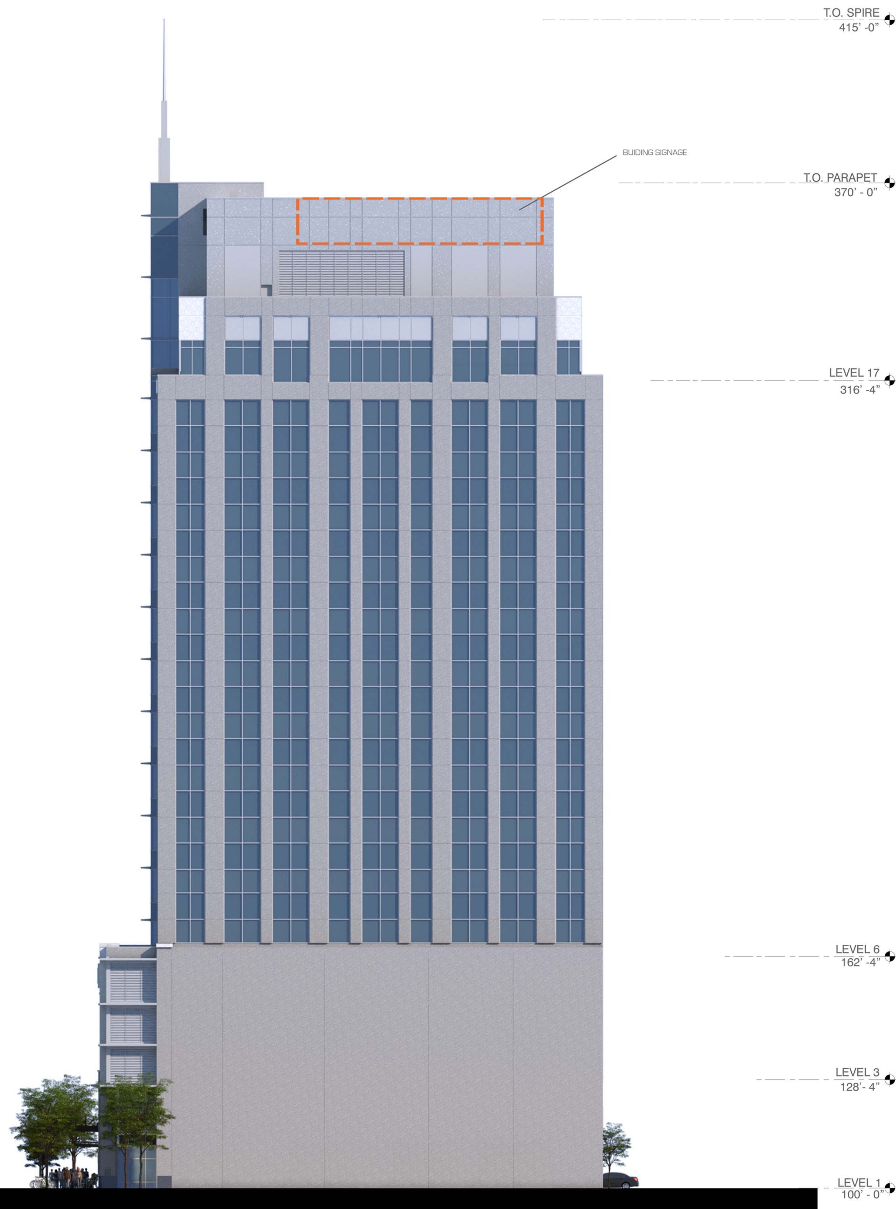
NORTH ELEVATION 1/16" = 1'
