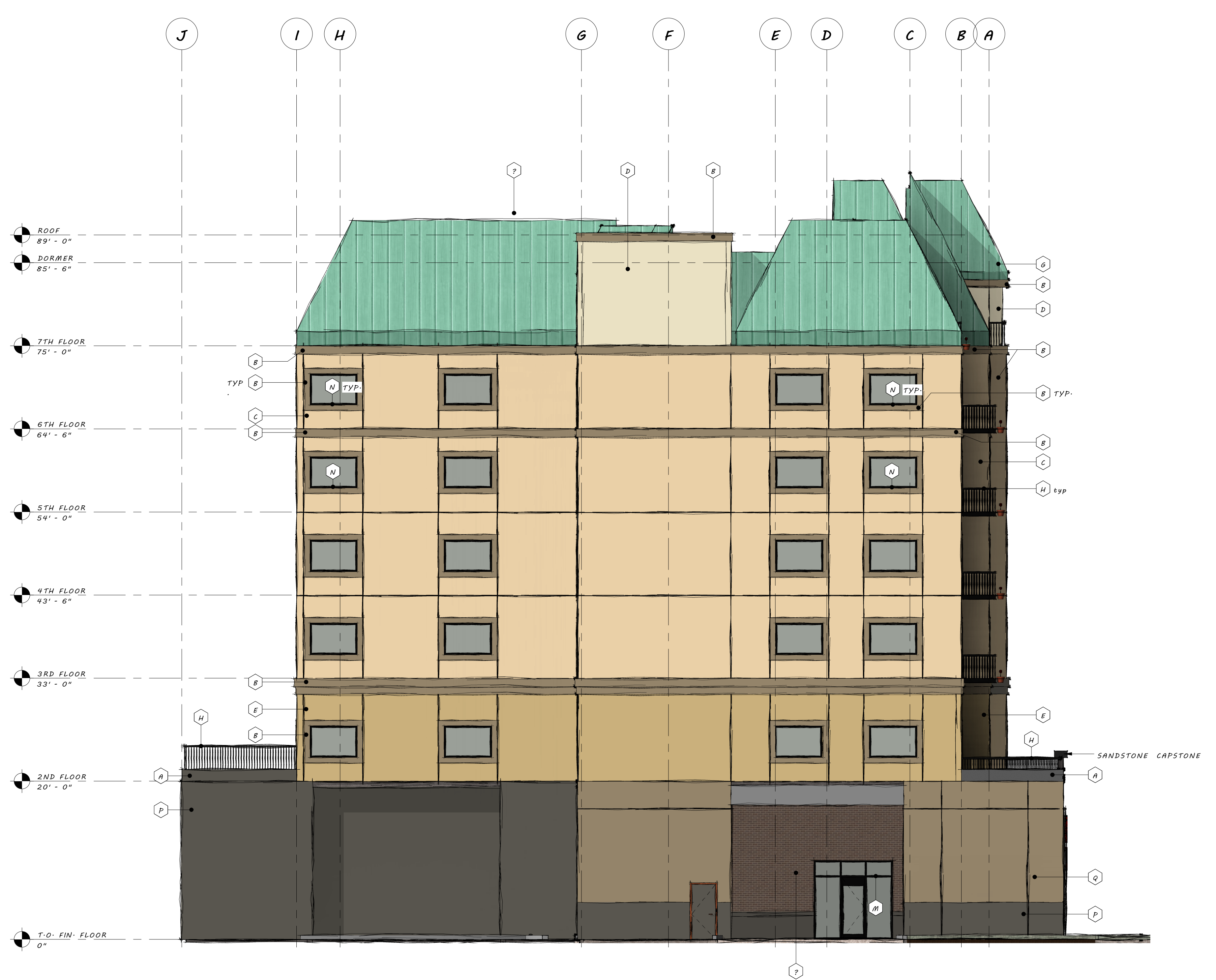
7 EAST ELEVATION 1/8" = 1'-0"
