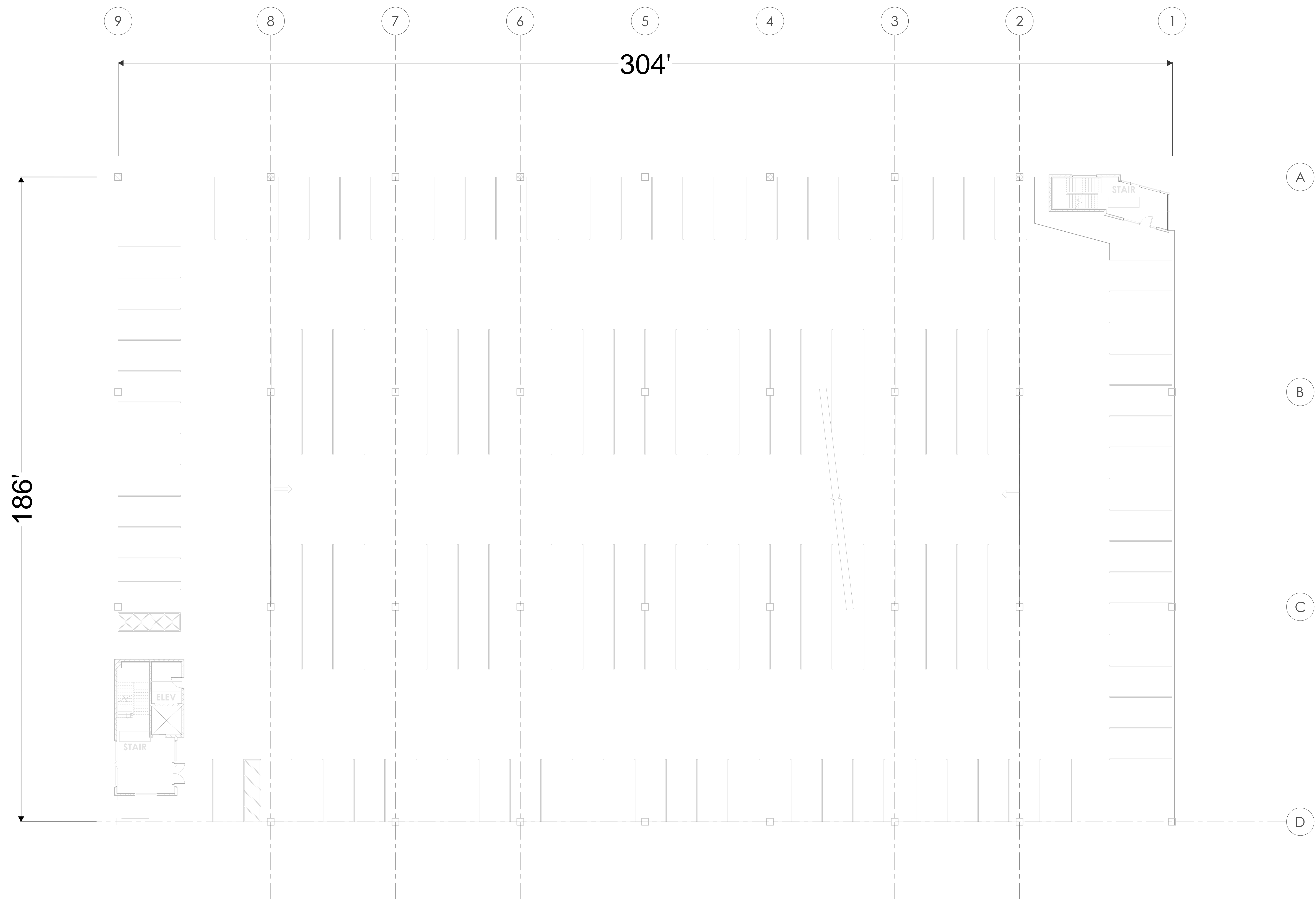
PARKING — LEVELS 2-3 178 STALLS
