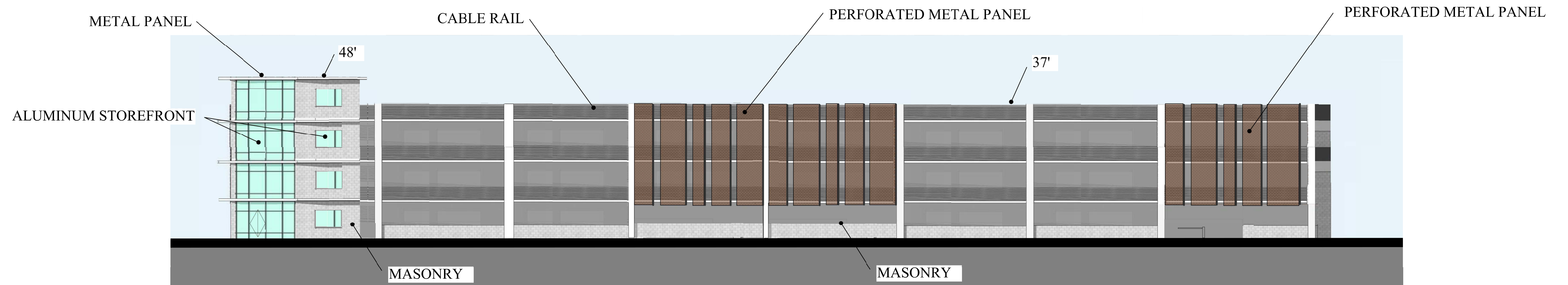
NORTH ELEVATION
