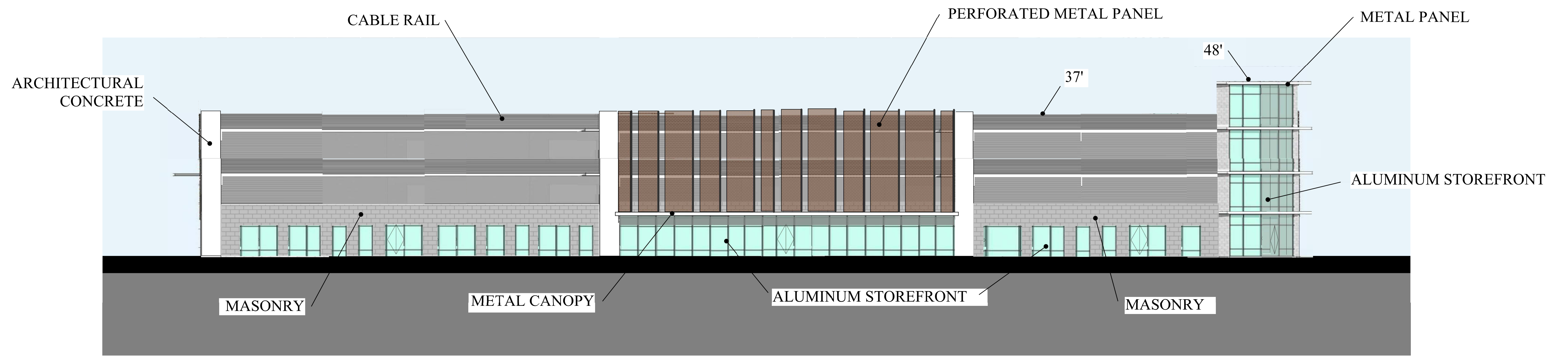
EAST ELEVATION
