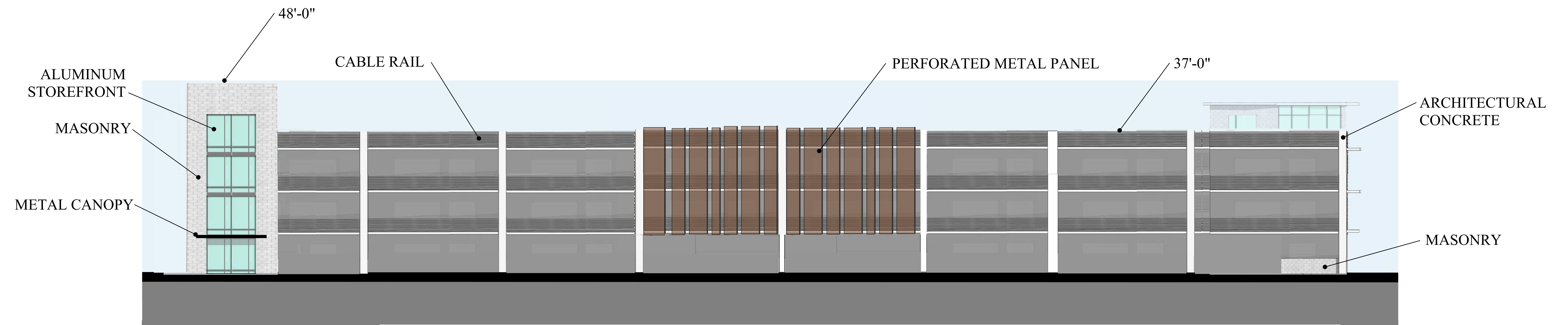
WEST ELEVATION
